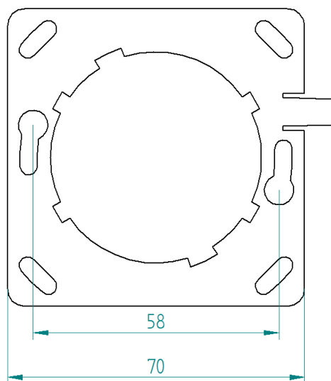
Figure 2 mounting plate
