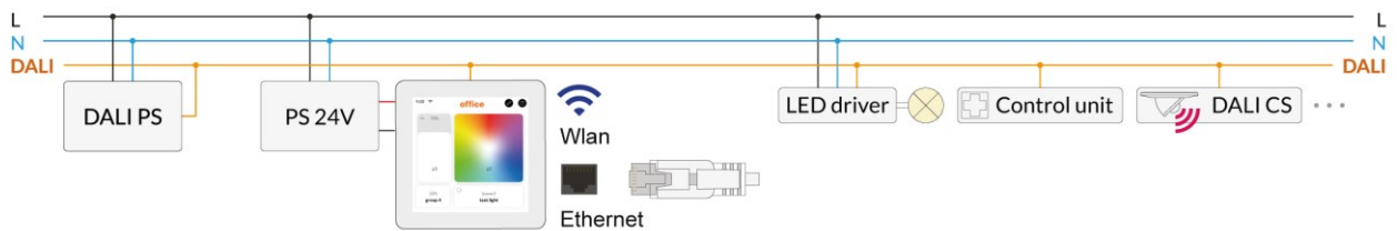
Figure 1 Typical Application
